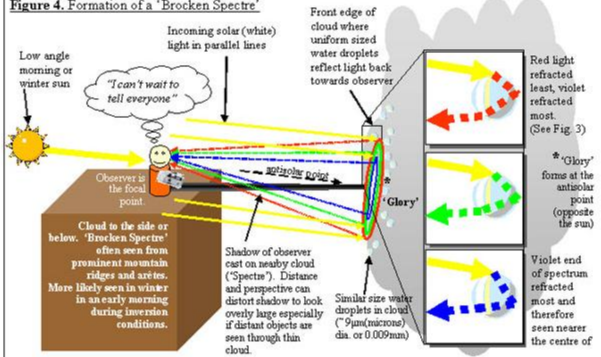
Fig. 4. Formation of a Broken Spectre by Peter Burgess
