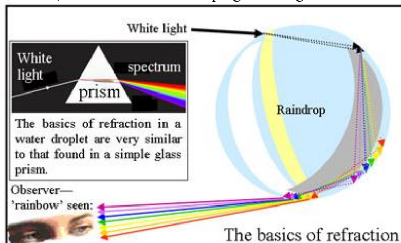
Fig 3. The Basics of Refraction
